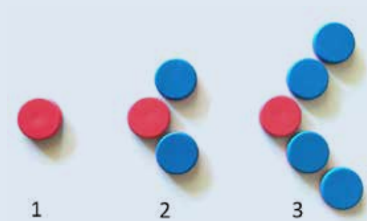
Figure 13. Aspect structural.
